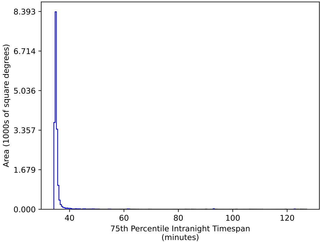
too_elab_r16_d2_giz_v3.4_10yrs WFD gr bands: 75th Percentile Intranight Timespan
