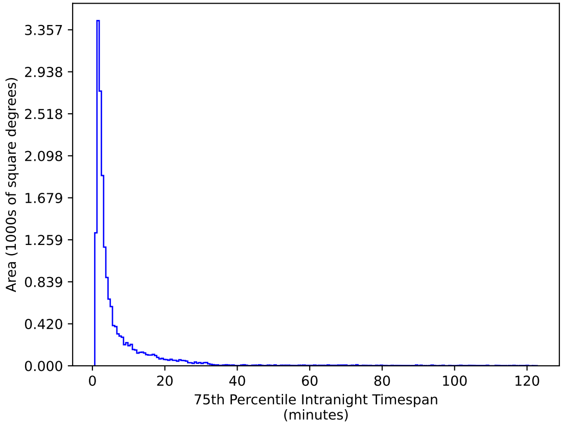
too_elab_r16_d2_giz_v3.4_10yrs WFD g band: 75th Percentile Intranight Timespan
