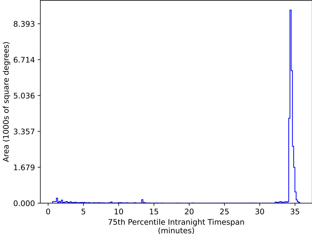
too_elab_r16_d2_giz_v3.4_10yrs All sky zy bands: 75th Percentile Intranight Timespan
