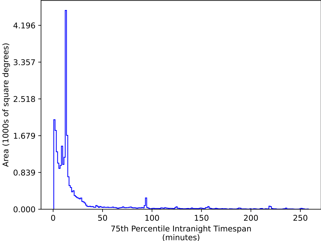
too_elab_r16_d2_giz_v3.4_10yrs All sky z band: 75th Percentile Intranight Timespan
