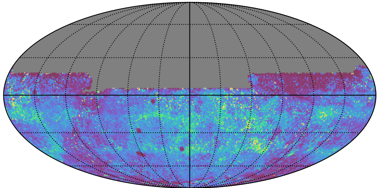
too_elab_r16_d2_giz_v3.4_10yrs All sky y band: 75th Percentile Intranight Timespan
