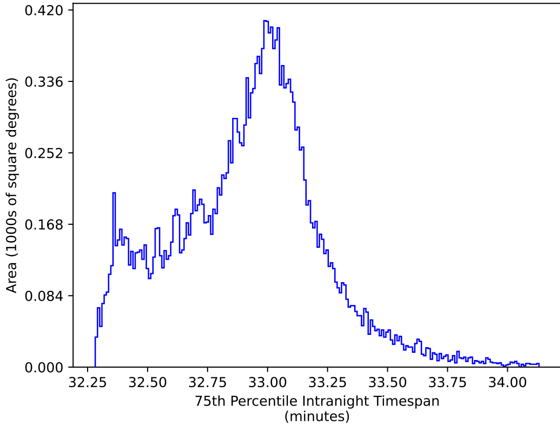
too_elab_r16_d2_giz_v3.4_10yrs All sky y band: 75th Percentile Intranight Timespan
