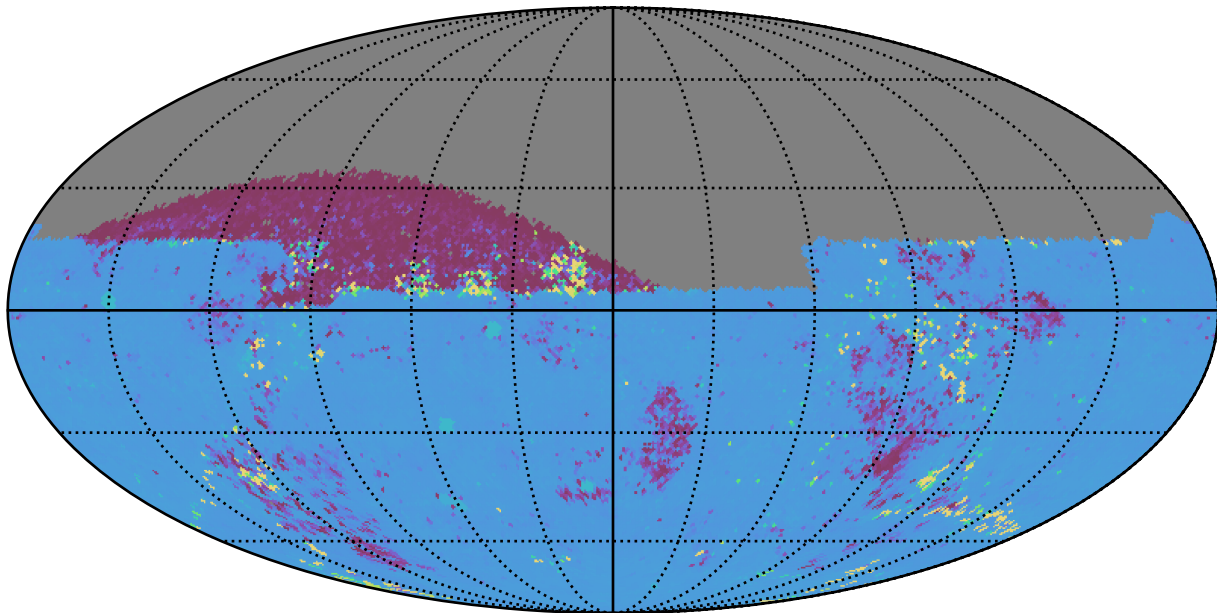
too_elab_r16_d2_giz_v3.4_10yrs All sky ug bands: 75th Percentile Intranight Timespan
