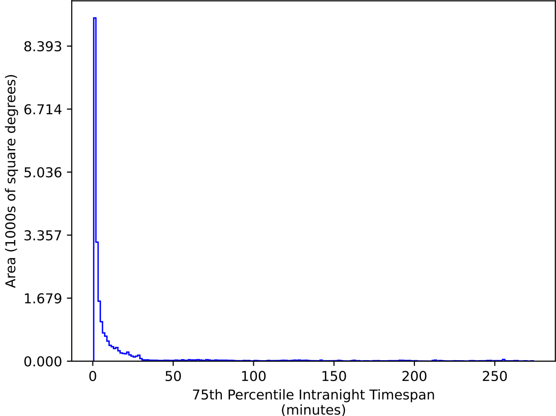
too_elab_r16_d2_giz_v3.4_10yrs All sky u band: 75th Percentile Intranight Timespan
