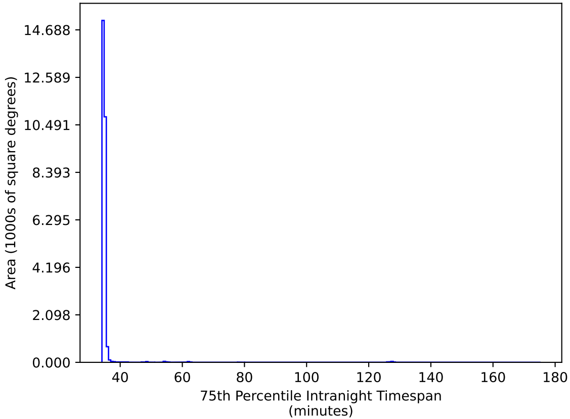
too_elab_r16_d2_giz_v3.4_10yrs All sky iz bands: 75th Percentile Intranight Timespan
