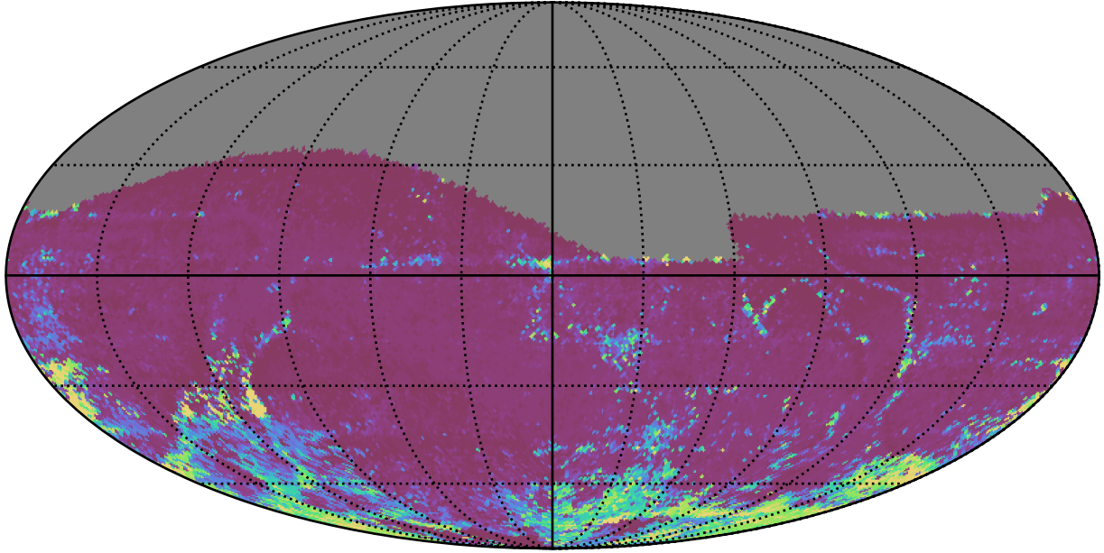
too_elab_r16_d2_giz_v3.4_10yrs All sky i band: 75th Percentile Intranight Timespan
