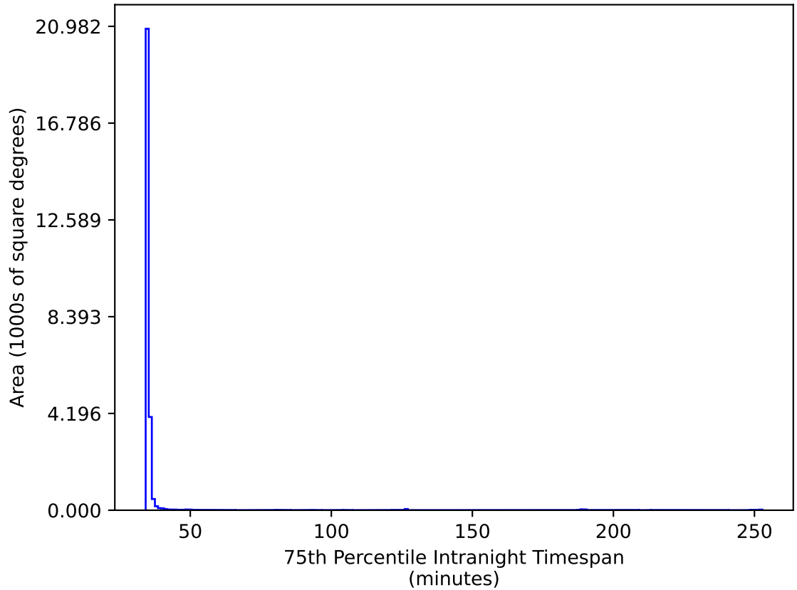
too_elab_r16_d2_giz_v3.4_10yrs All sky gr bands: 75th Percentile Intranight Timespan
