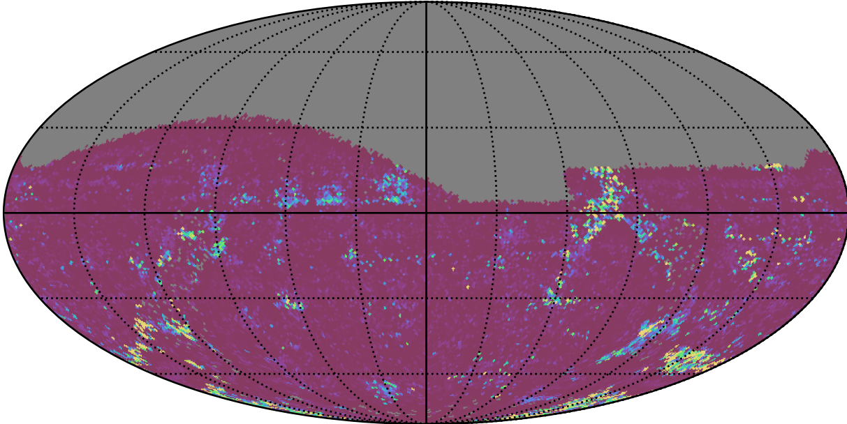
too_elab_r16_d2_giz_v3.4_10yrs All sky g band: 75th Percentile Intranight Timespan
