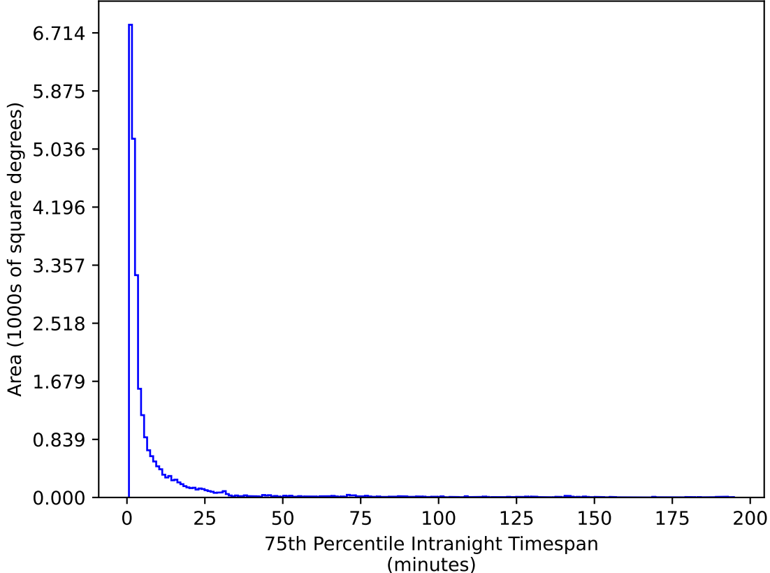
too_elab_r16_d2_giz_v3.4_10yrs All sky g band: 75th Percentile Intranight Timespan
