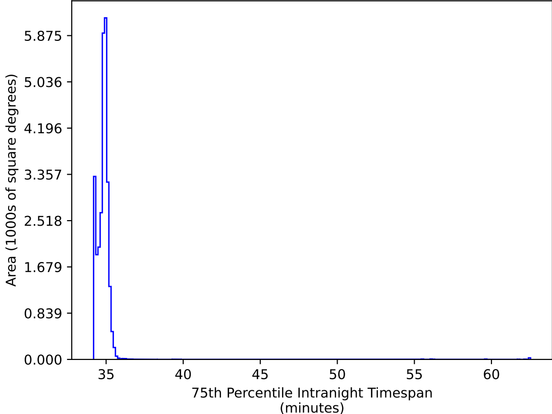
too_elab_r16_d2_giz_v3.4_10yrs All sky all bands: 75th Percentile Intranight Timespan
