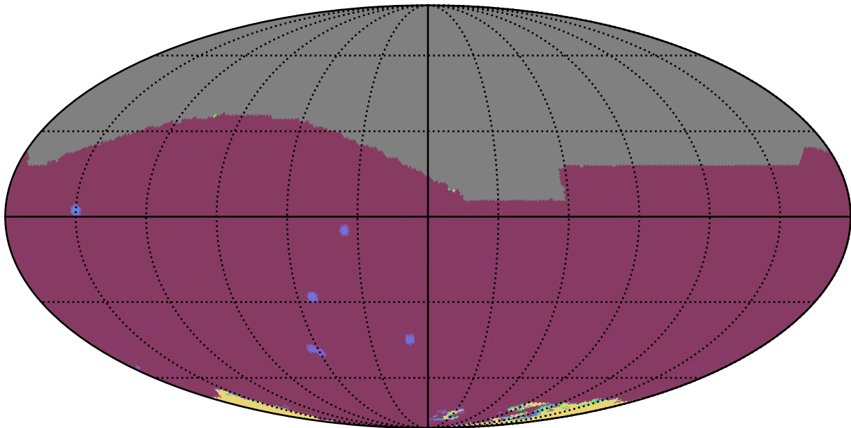
too_elab_r16_d2_giz_v3.4_10yrs All sky: 75th Percentile Intranight Timespan
