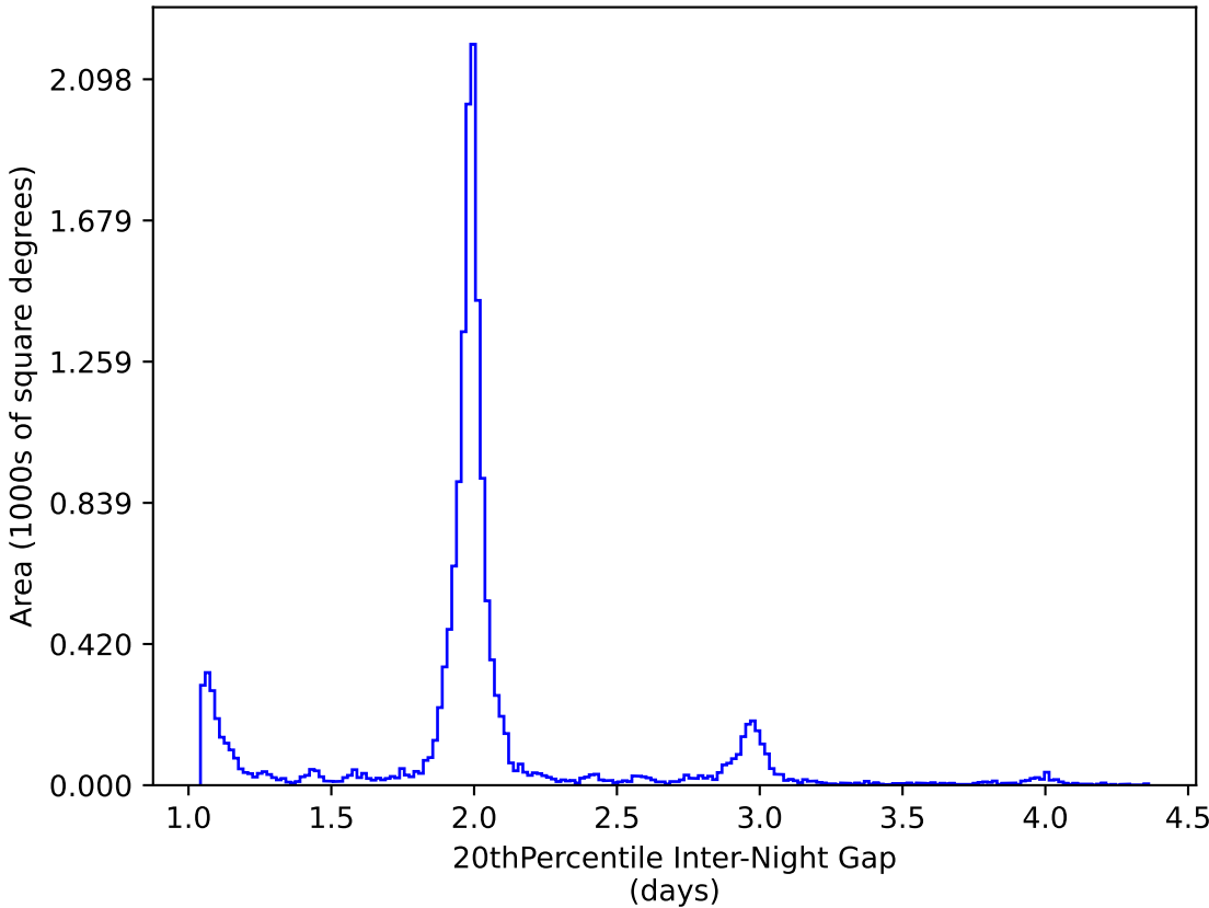
too_elab_r16_d2_giz_v3.4_10yrs WFD y band: 20thPercentile Inter-Night Gap
