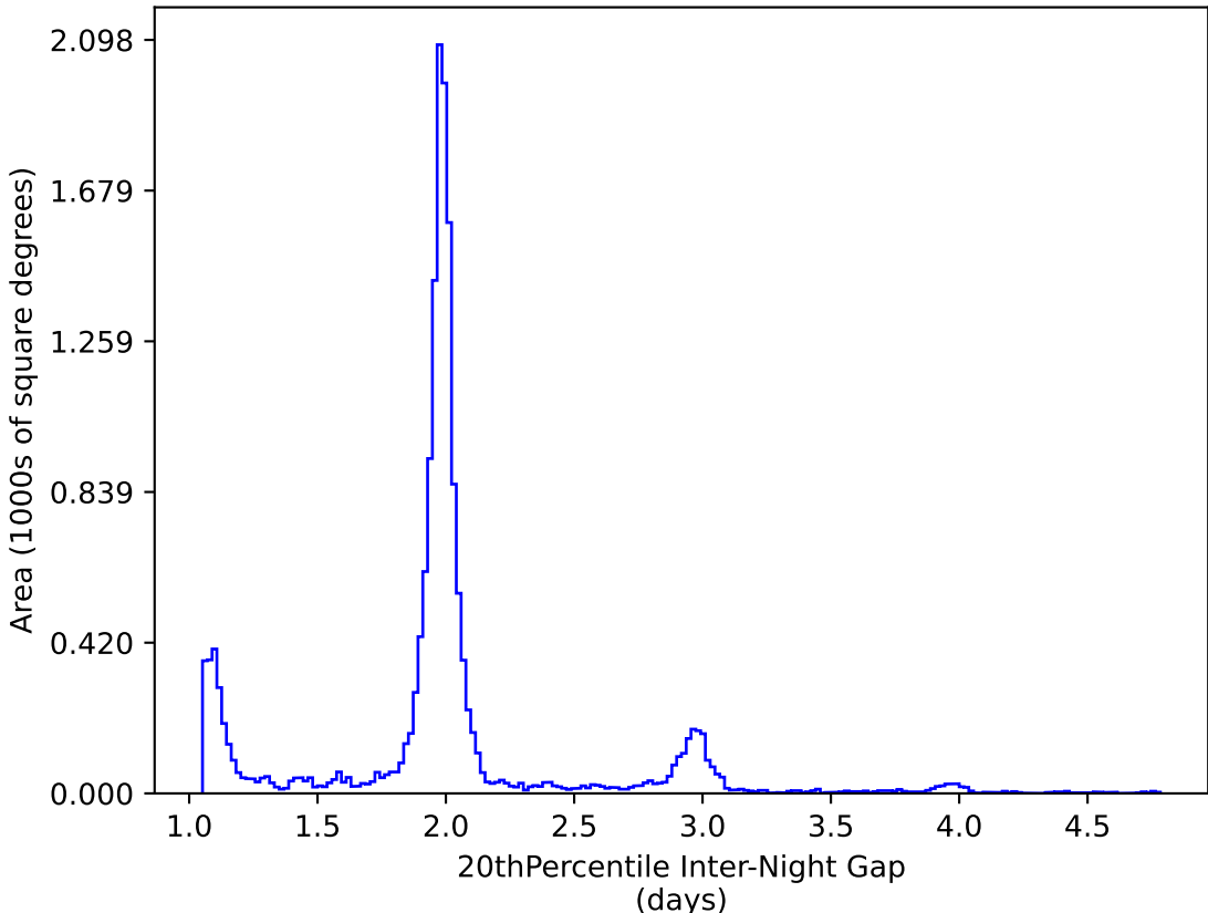
too_elab_r16_d2_giz_v3.4_10yrs WFD y band: 20thPercentile Inter-Night Gap
