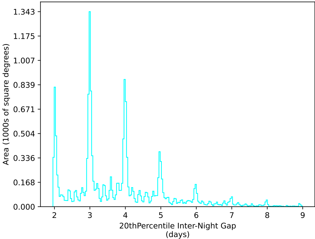
too_elab_r16_d2_giz_v3.4_10yrs WFD u band: 20thPercentile Inter-Night Gap
