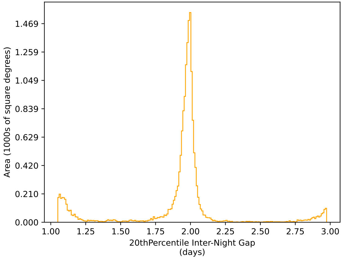
too_elab_r16_d2_giz_v3.4_10yrs WFD r band: 20thPercentile Inter-Night Gap
