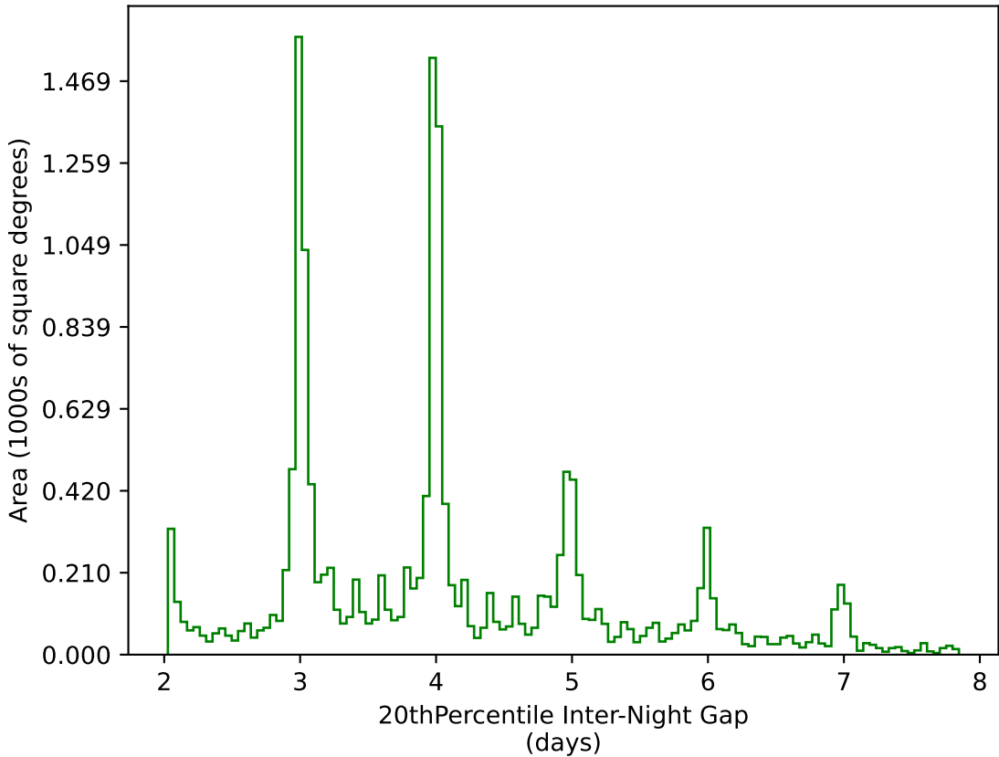
too_elab_r16_d2_giz_v3.4_10yrs WFD g band: 20thPercentile Inter-Night Gap
