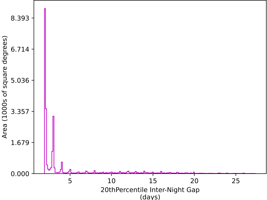
too_elab_r16_d2_giz_v3.4_10yrs All sky z band: 20thPercentile Inter-Night Gap
