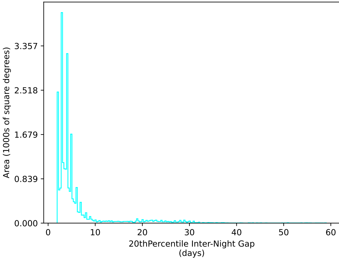
too_elab_r16_d2_giz_v3.4_10yrs All sky u band: 20thPercentile Inter-Night Gap
