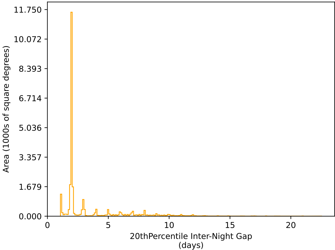
too_elab_r16_d2_giz_v3.4_10yrs All sky r band: 20thPercentile Inter-Night Gap
