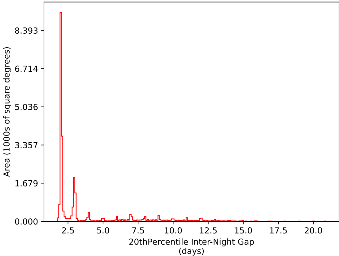
too_elab_r16_d2_giz_v3.4_10yrs All sky i band: 20thPercentile Inter-Night Gap
