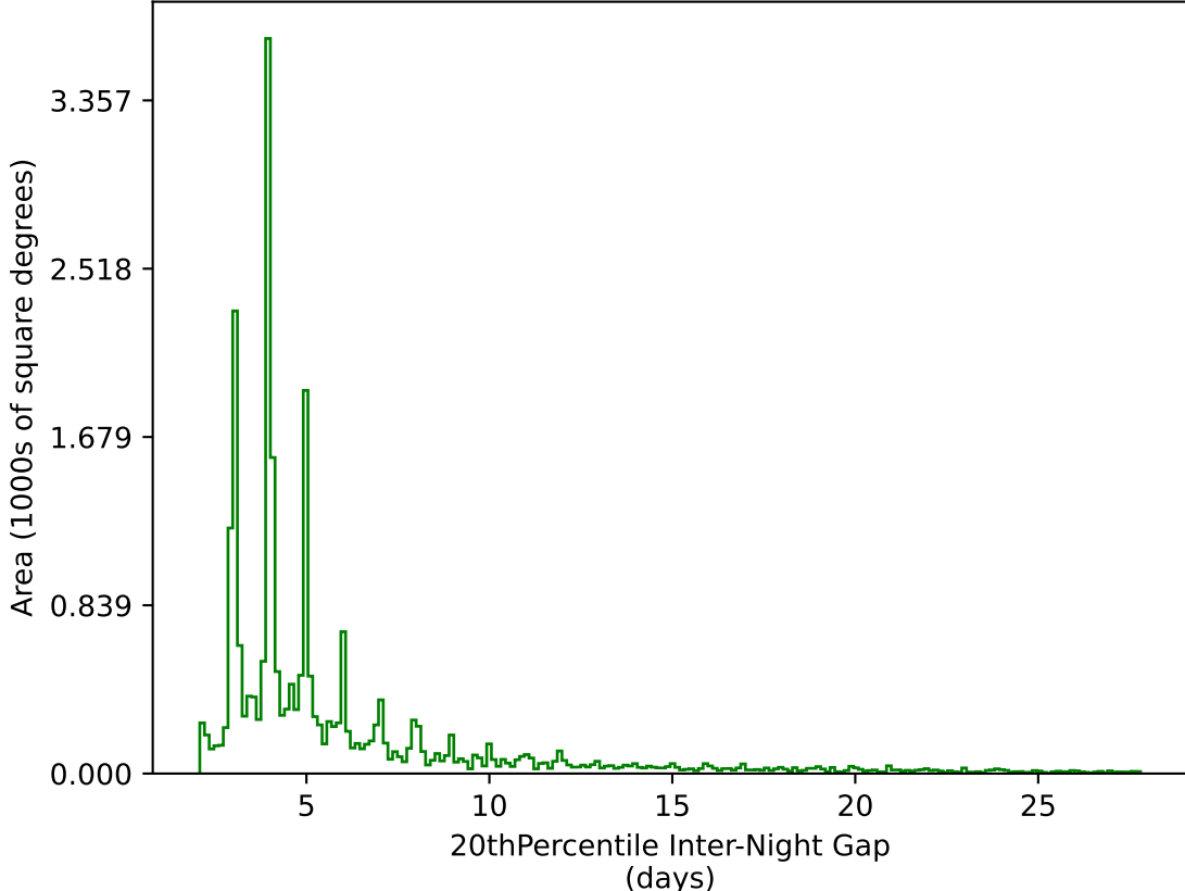
too_elab_r16_d2_giz_v3.4_10yrs All sky g band: 20thPercentile Inter-Night Gap
