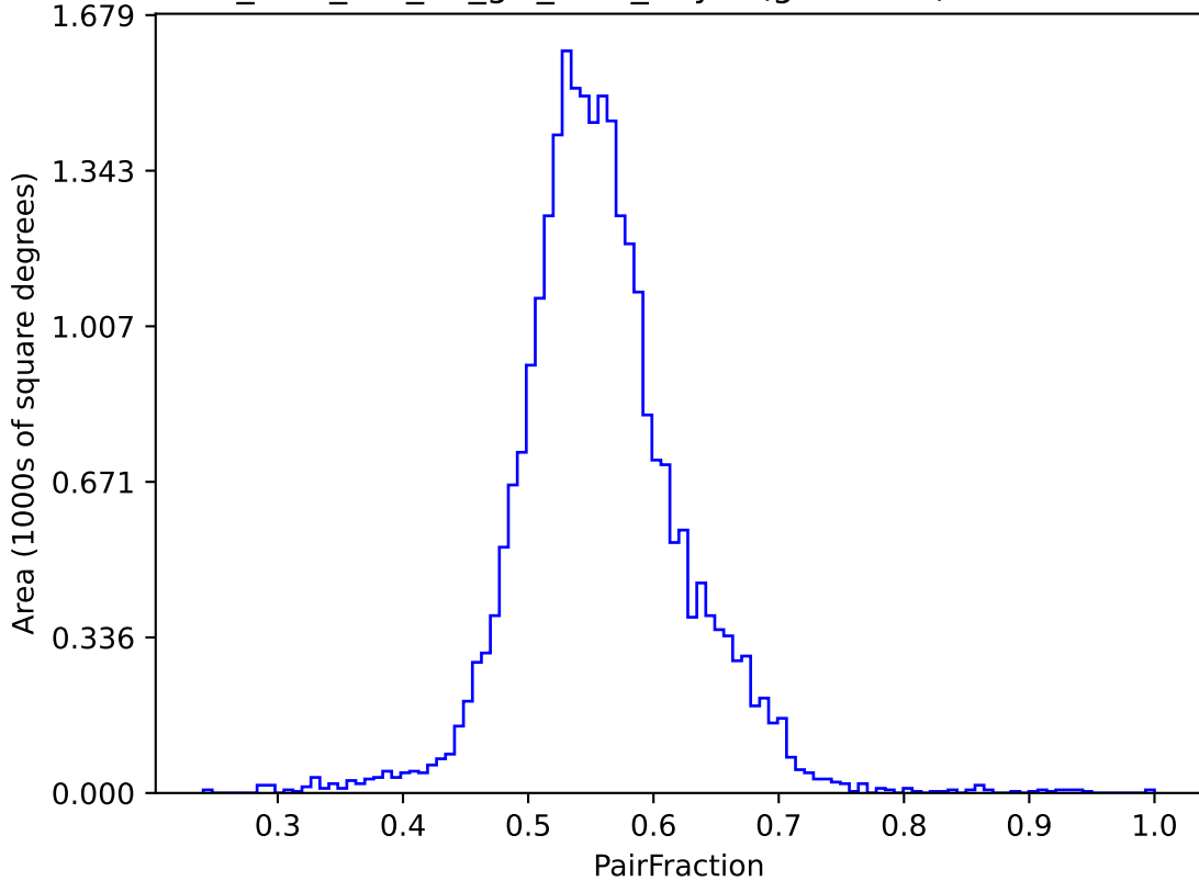
too_elab_r16_d2_giz_v3.4_10yrs (g or r or i): PairFraction
