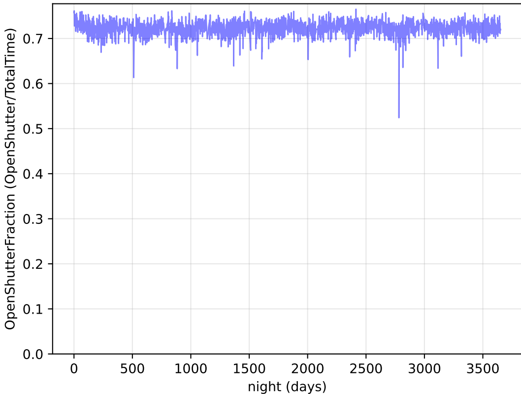
too_elab_r16_d2_giz_v3.4_10yrs : OpenShutterFraction
