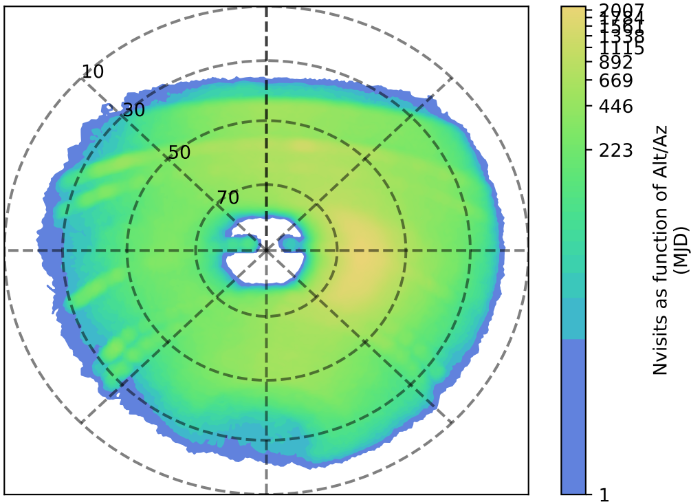
too_elab_r16_d2_giz_v3.4_10yrs y: Nvisits as function of Alt/Az
