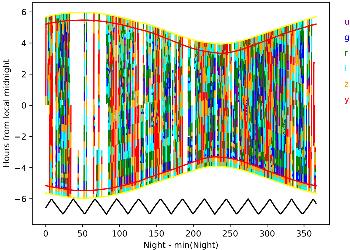
too_elab_r16_d2_giz_v3.4_10yrs year 3-4: Hourglass
