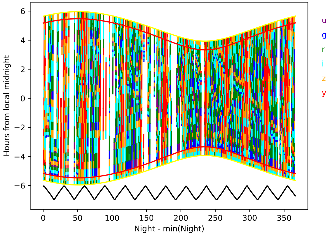
too_elab_r16_d2_giz_v3.4_10yrs year 1-2: Hourglass
