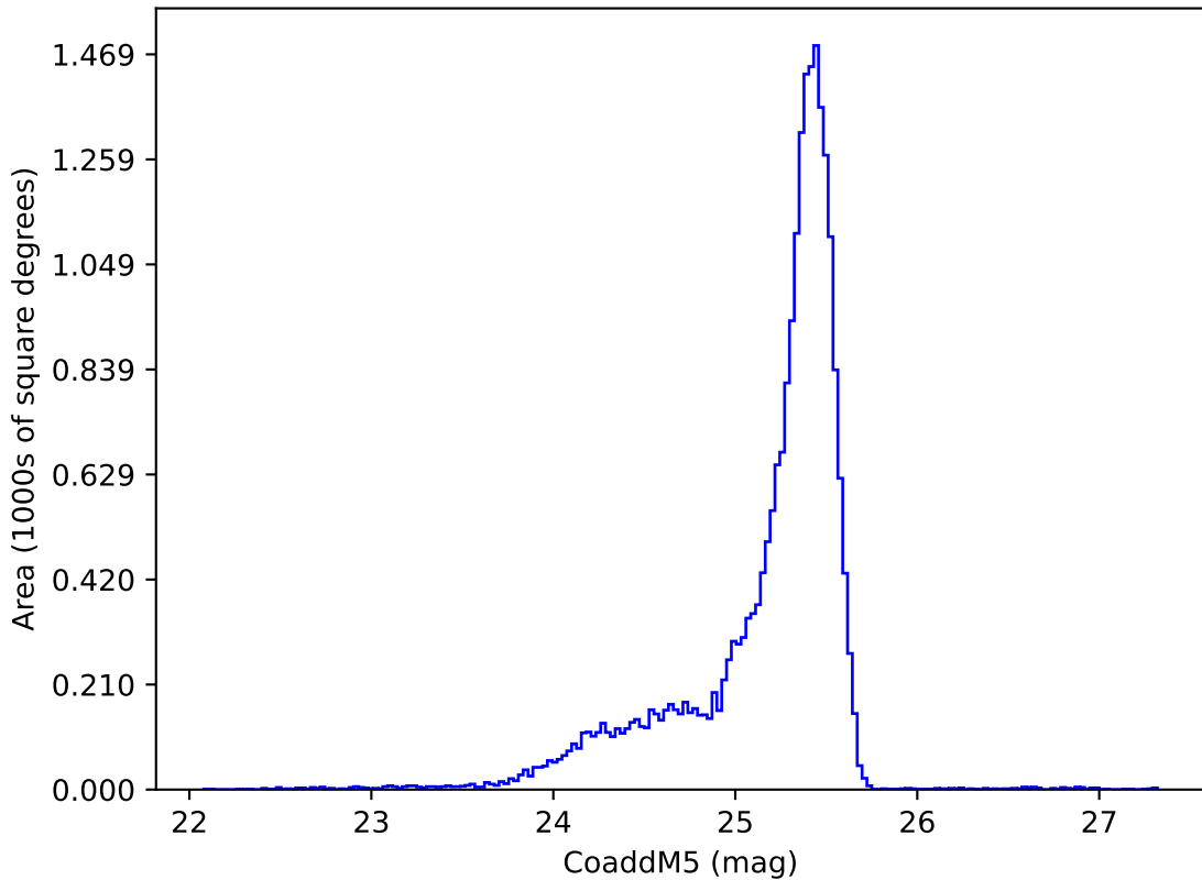
too_elab_r16_d2_giz_v3.4_10yrs u: CoaddM5
