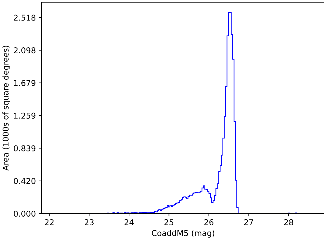
too_elab_r16_d2_giz_v3.4_10yrs i: CoaddM5
