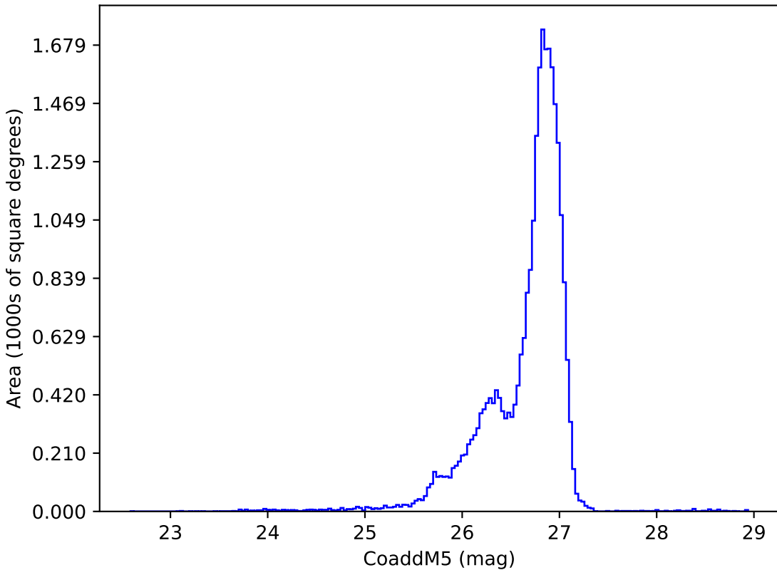
too_elab_r16_d2_giz_v3.4_10yrs g: CoaddM5
