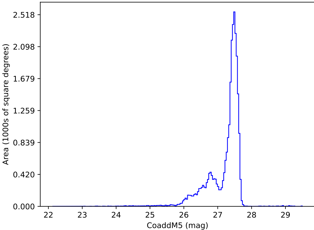
too_elab_r16_d2_giz_v3.4_10yrs : CoaddM5
