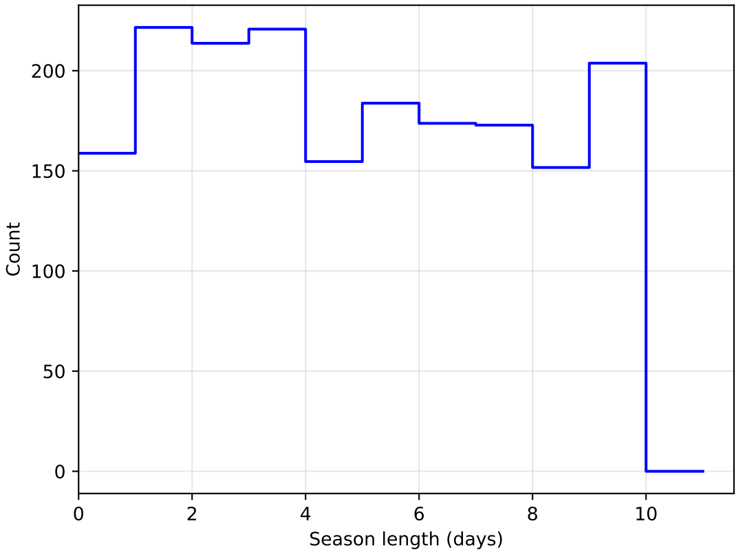
too_elab_r16_d2_giz_v3.4_10yrs DD:WFD all bands: SeasonLength
