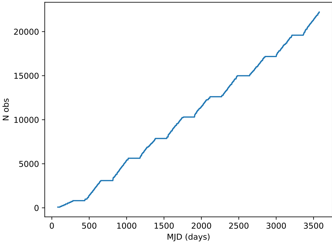
too_elab_r16_d2_giz_v3.4_10yrs all bands: DD:XMM_LSS Cumulative NVisits
