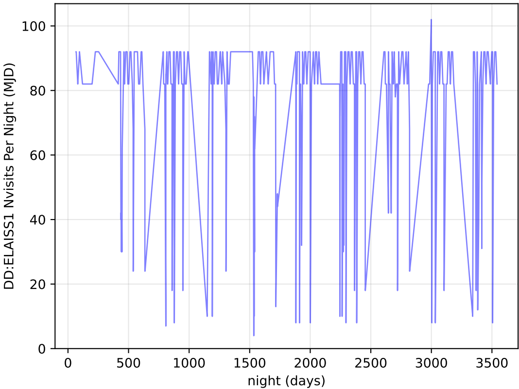
too_elab_r16_d2_giz_v3.4_10yrs all bands: DD:ELAISS1 Nvisits Per Night
