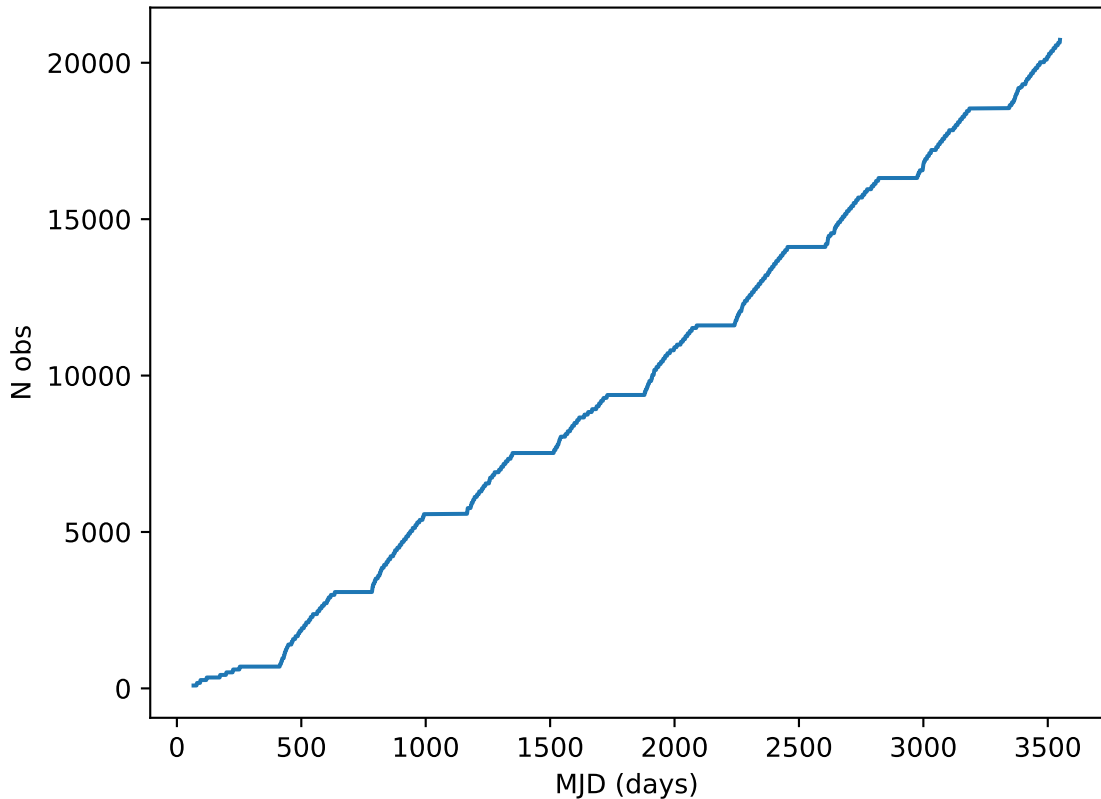
too_elab_r16_d2_giz_v3.4_10yrs all bands: DD:ELAISS1 Cumulative NVisits
