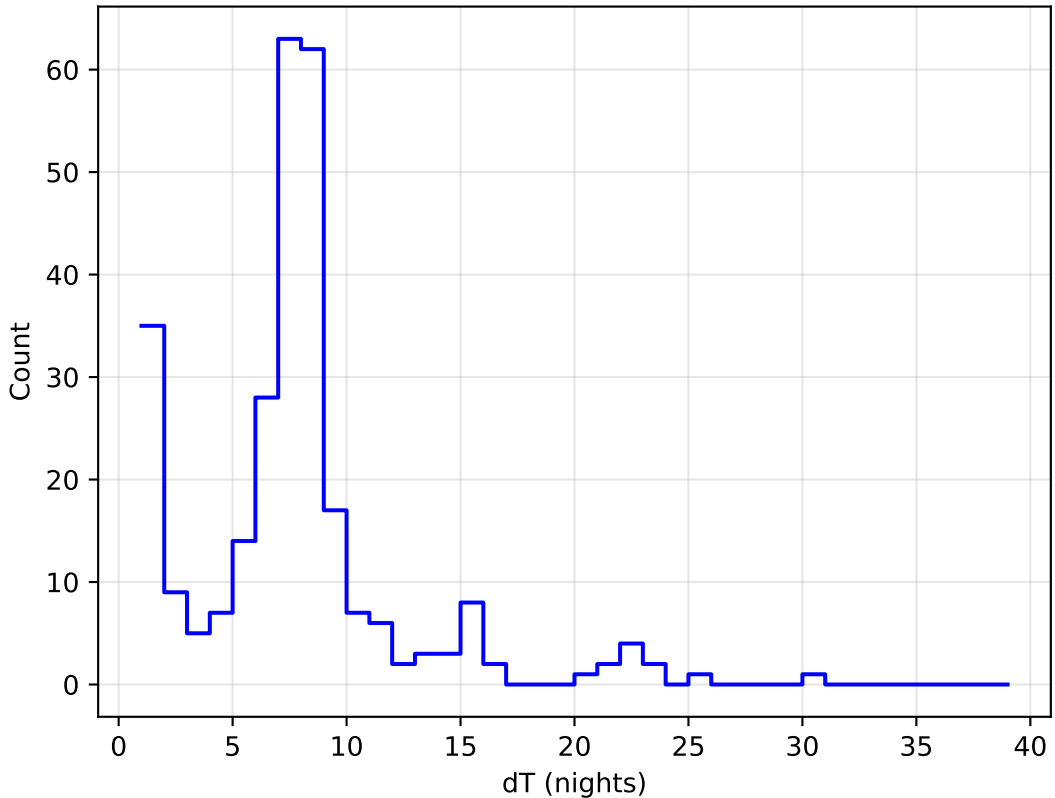
too_elab_r16_d2_giz_v3.4_10yrs all bands: DD:ECDFS Delta Nights Histogram
