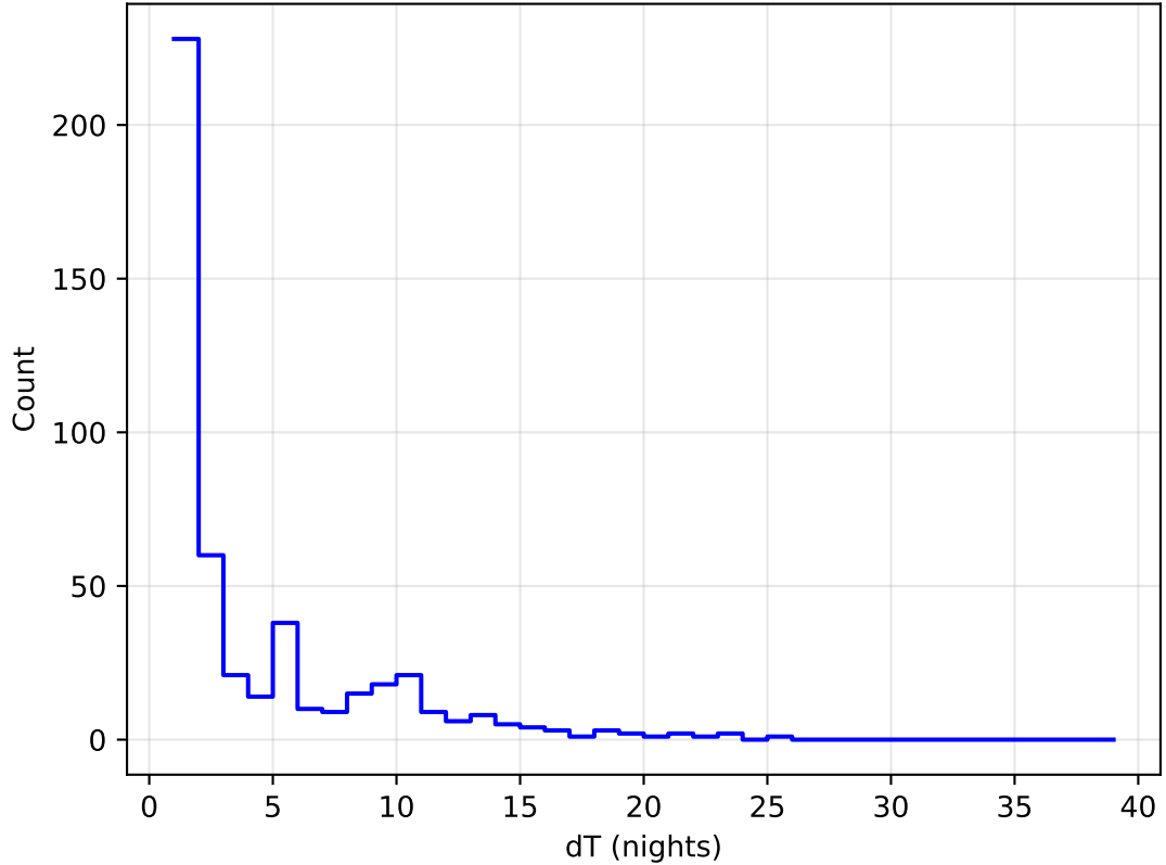
too_elab_r16_d2_giz_v3.4_10yrs all bands: DD: COSMOS Delta Nights Histogram
