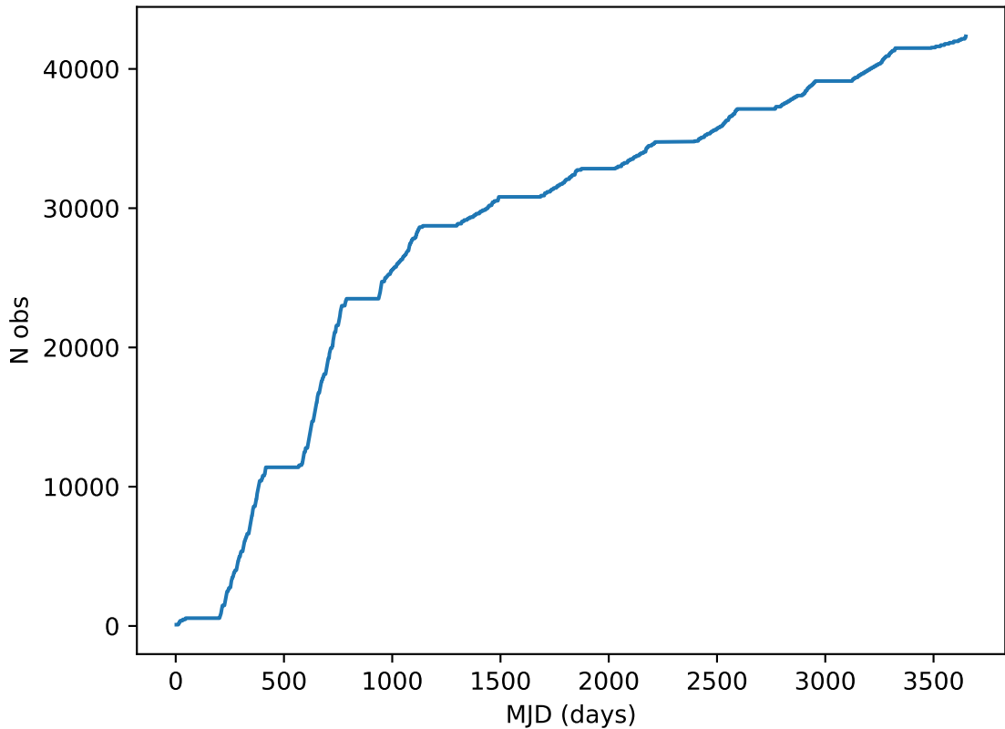
too_elab_r16_d2_giz_v3.4_10yrs all bands: DD: COSMOS Cumulative NVisits
