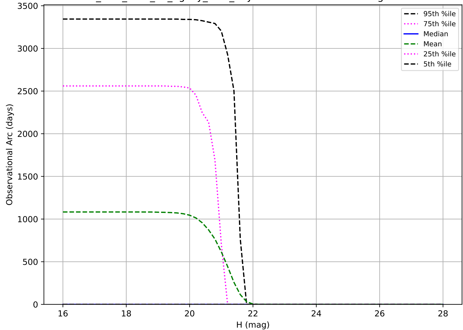
too_elab_r128_d3_ugrizy_v3.4_10yrs: Observational Arc Length Vatira
