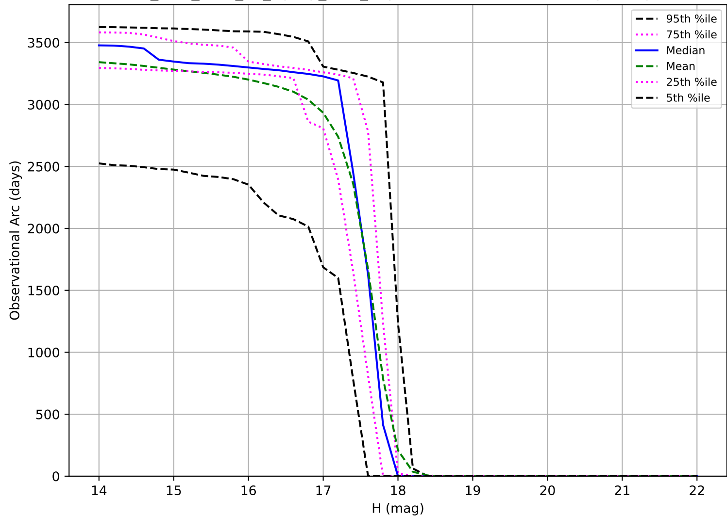
too_elab_r128_d3_ugrizy_v3.4_10yrs: Observational Arc Length Trojan
