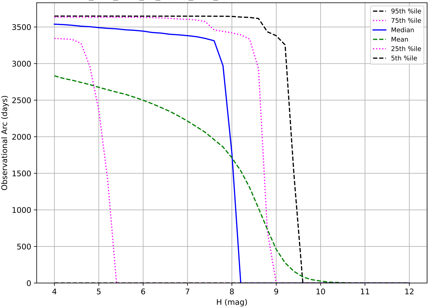
too_elab_r128_d3_ugrizy_v3.4_10yrs: Observational Arc Length TNO
