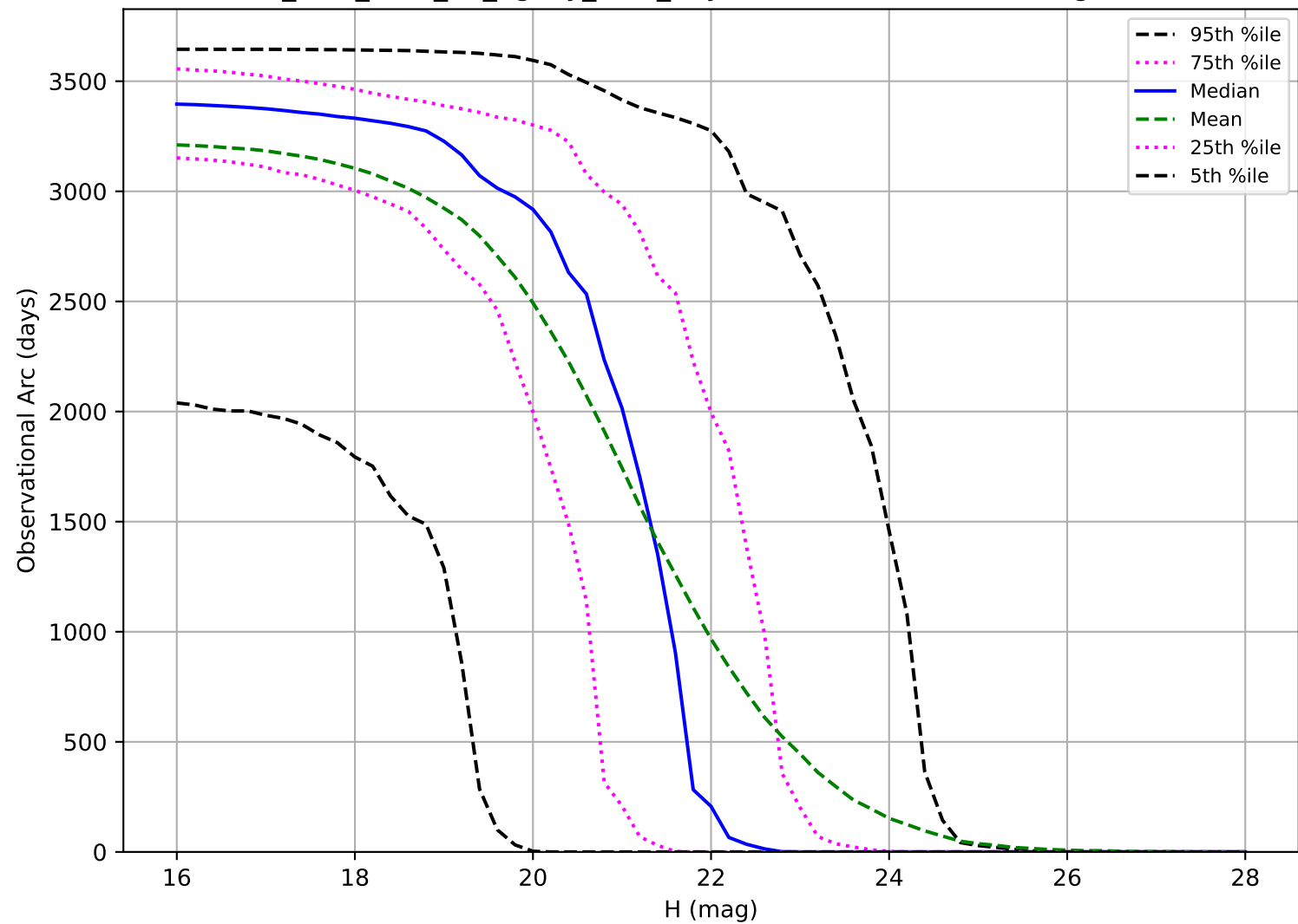
too_elab_r128_d3_ugrizy_v3.4_10yrs: Observational Arc Length PHA
