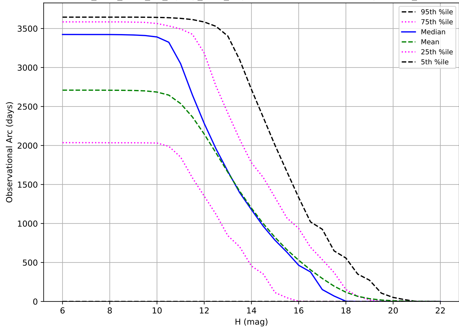
too_elab_r128_d3_ugrizy_v3.4_10yrs: Observational Arc Length OCC_r5
