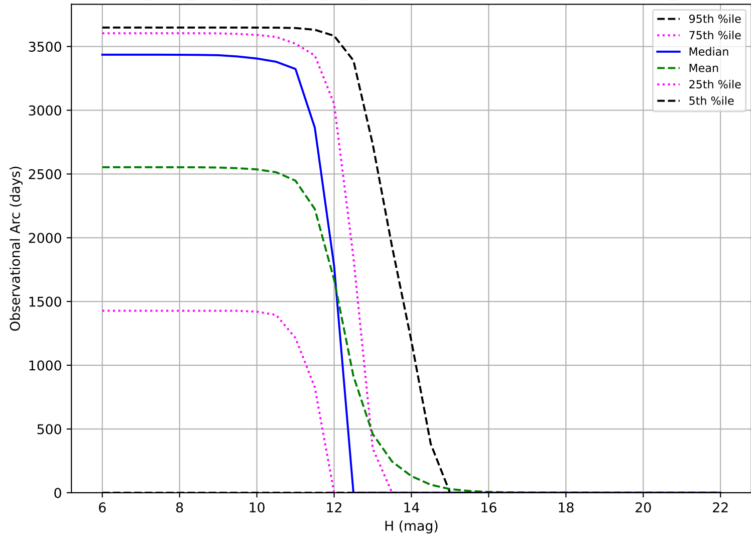
too_elab_r128_d3_ugrizy_v3.4_10yrs: Observational Arc Length OCC_r20
