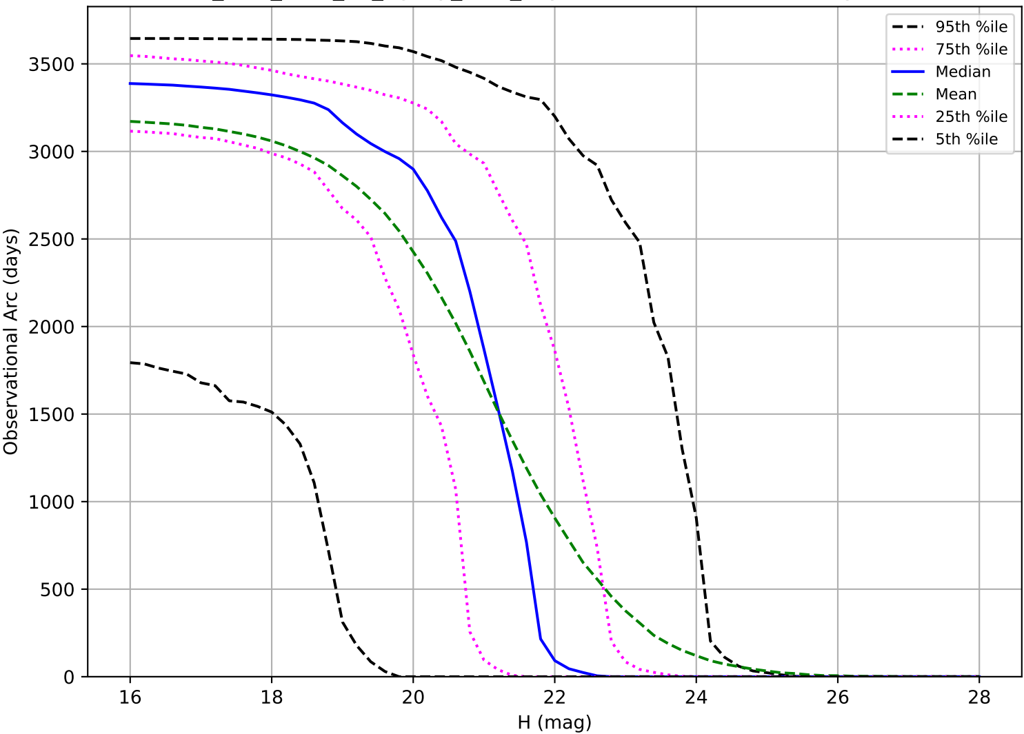
too_elab_r128_d3_ugrizy_v3.4_10yrs: Observational Arc Length NEO
