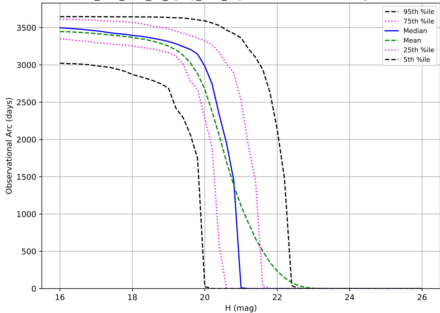
too_elab_r128_d3_ugrizy_v3.4_10yrs: Observational Arc Length MBA
