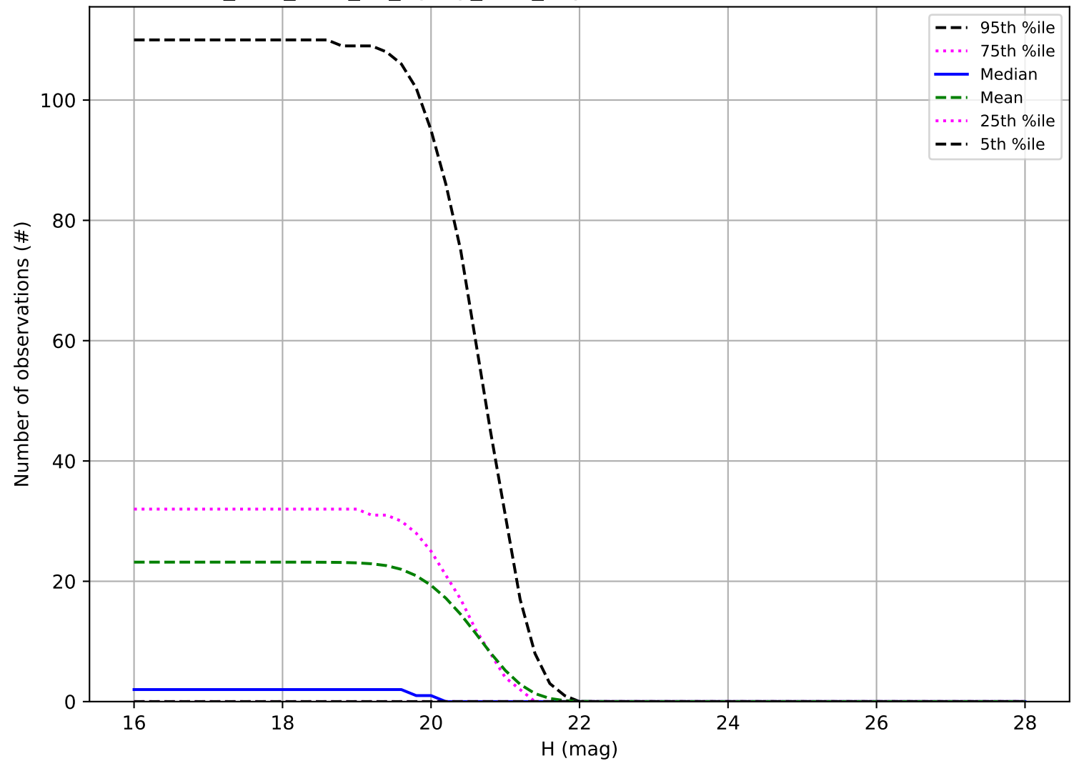
too_elab_r128_d3_ugrizy_v3.4_10yrs: Number of observations Vatira
