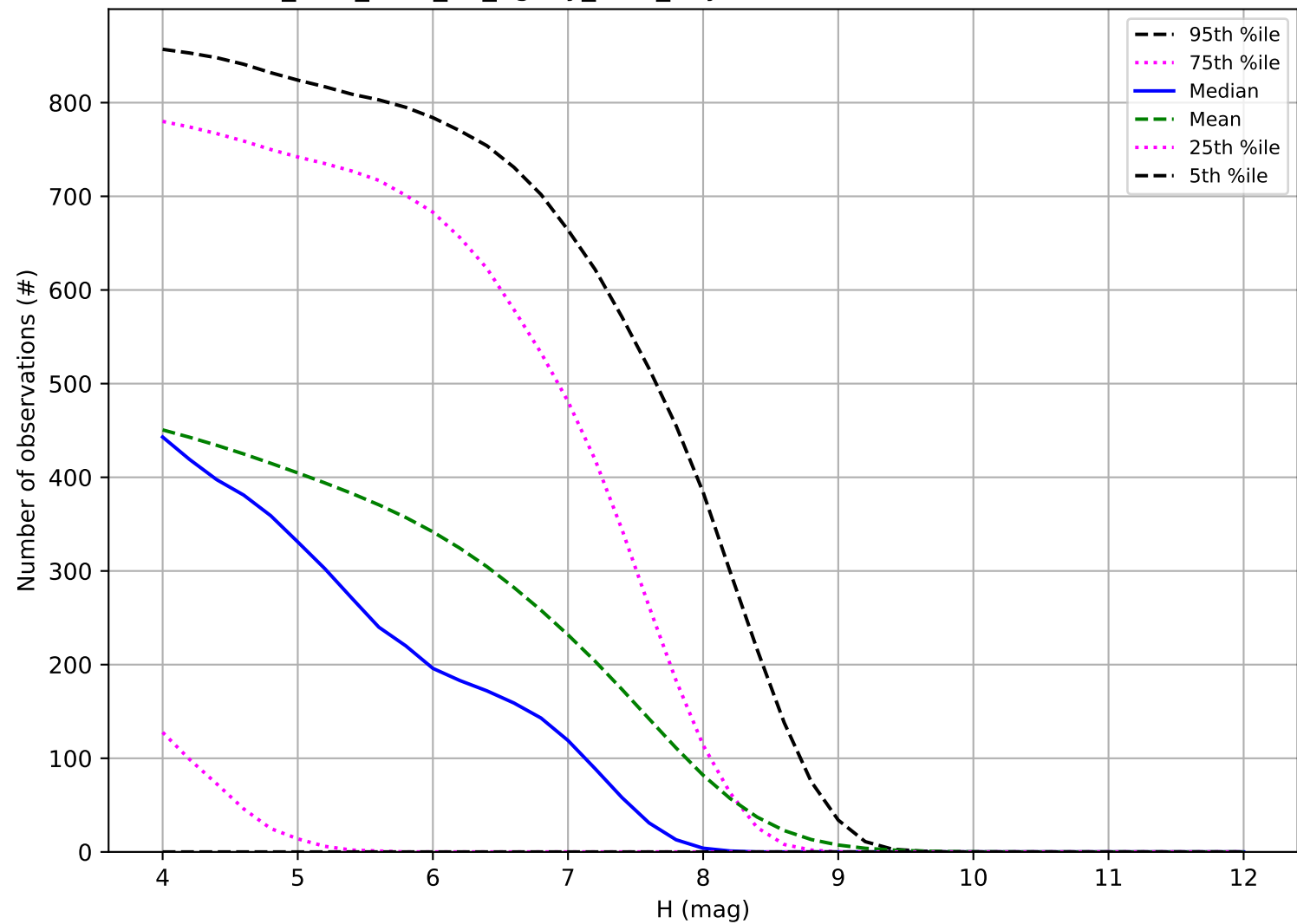
too_elab_r128_d3_ugrizy_v3.4_10yrs: Number of observations TNO
